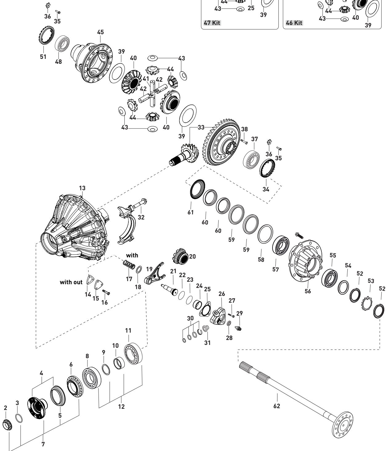
Axle with Ring Gear Ø 440mm R 440-13A/C22.5 Locked Differential
