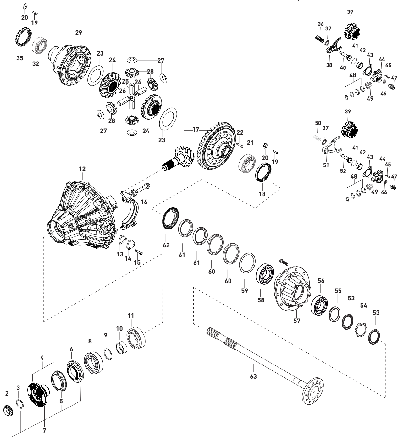
Axle with Ring Gear Ø 434,5 / 436,6 / 439,5mm Locked Differential
