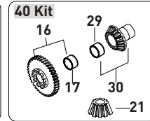
HD 7+ HL 7 INTERMEDIATE REAR Big Differential Axle with Ring Gear Ø 300 mm
