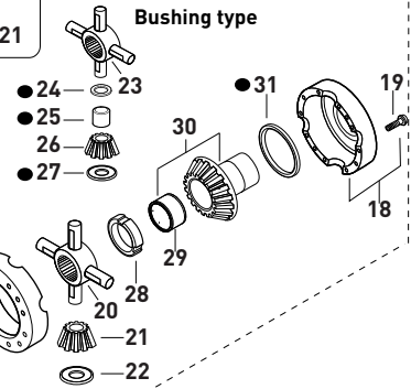
HD 7+ HL 7 INTERMEDIATE REAR Big Differential Axle with Ring Gear Ø 300 mm
